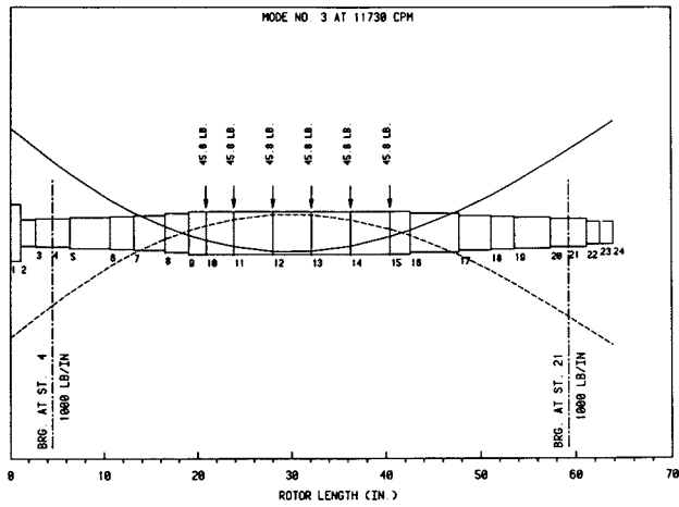
Figure 9. Calculated First Free-Free Mode.
