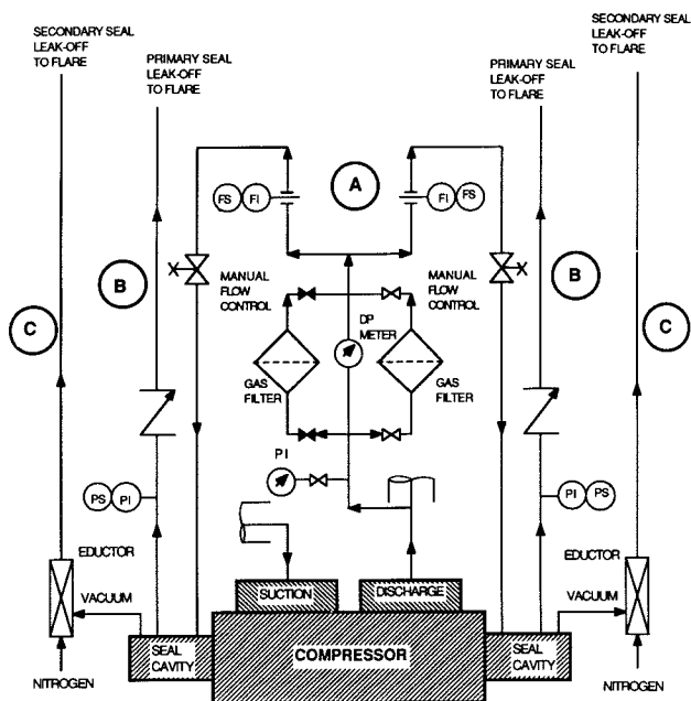
Figure 21. Gas Seal System Auxiliary Piping.
