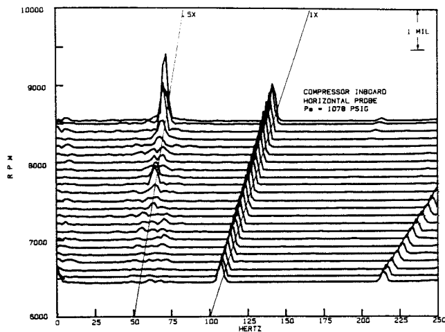
Figure 4. Cascade Plot at Suction Pressure = 1078 PSI.
