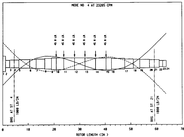
Figure 11. Calculated Second Free-Free Mode.
