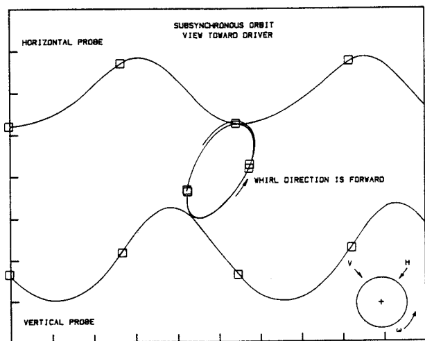
Figure 3. Subsynchronous Orbit Showing Forward Whirl.
