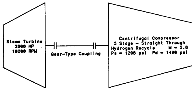
Figure 1. System Schematic.
