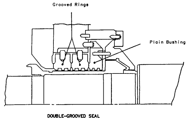
Figure 17. Double Grooved Oil Ring Seal.
