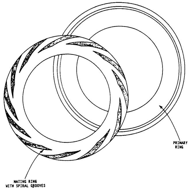
Figure 20. Surface Treatment of Primary and Mating Seal Rings.
