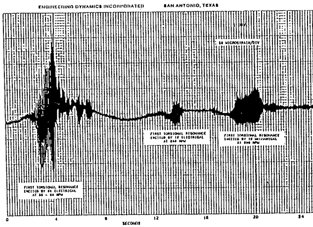
Figure 43. Strain Measurement on Gear Shaft During Runup.
