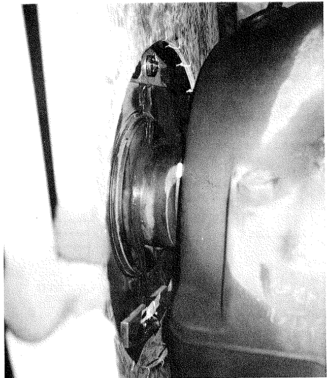
Figure 37. Rotating Transmitter and Batteries Installed on Coupling.
