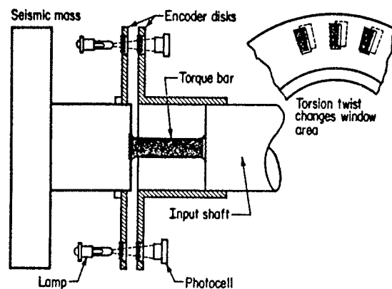
Figure 30. Torsional Measurement Using Photocells and Encoder Disk.
