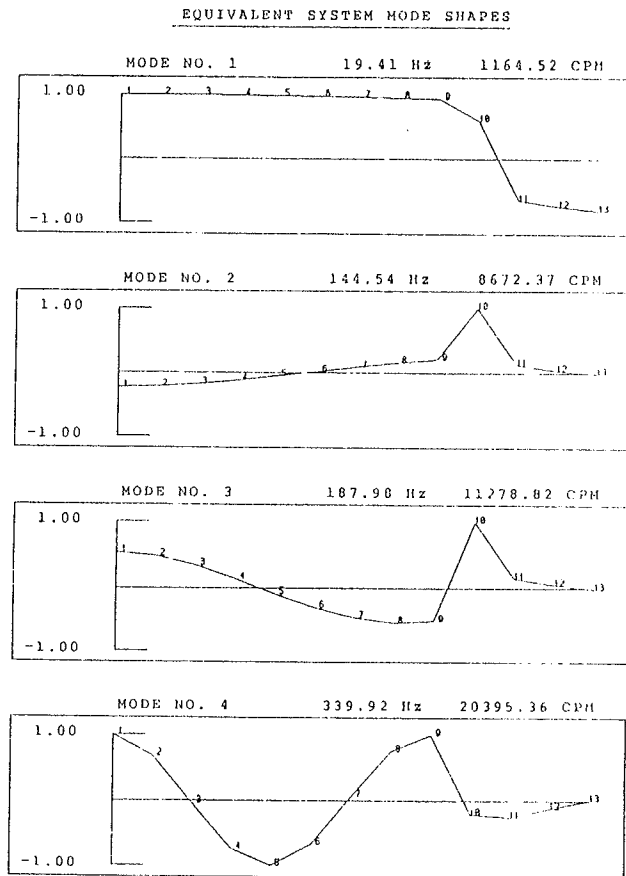
Figure 1. Torsional Natural Frequencies and Mode Shapes.
