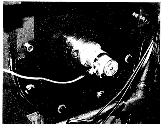
Figure 26. Torsiógraph Attached to Compressor Crankshaft.
