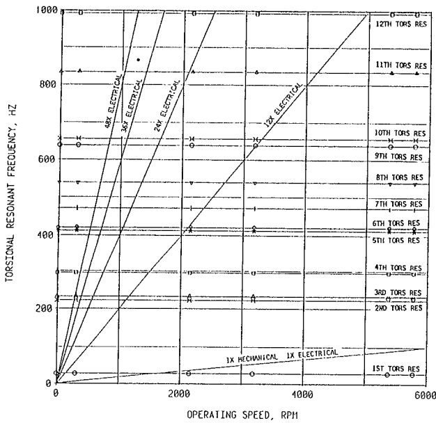
Figure 9. Interference Diagram of Centrifugal Compressor Train.
