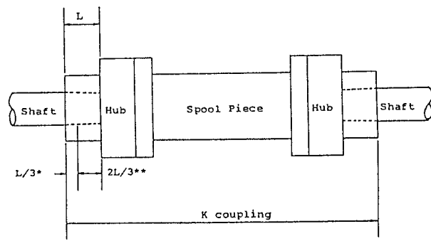
Figure 7. Coupling Shaft Penetration Assumption.
