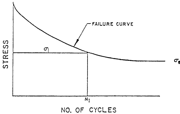
Figure 23. Cumulative Fatigue.
