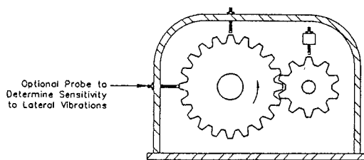
Figure 28. FM Torsional Pickups Installed on Gearset.
