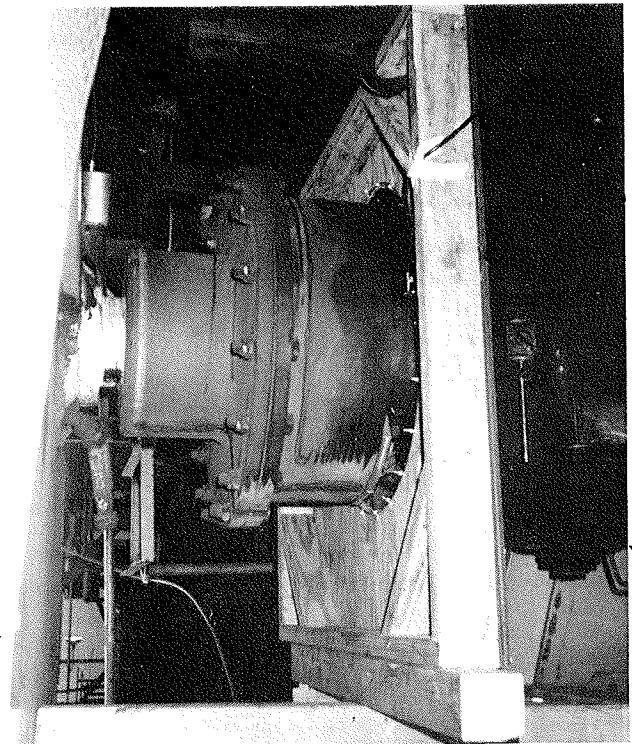
Figure 38. Stationary Antenna Support Around Coupling.
