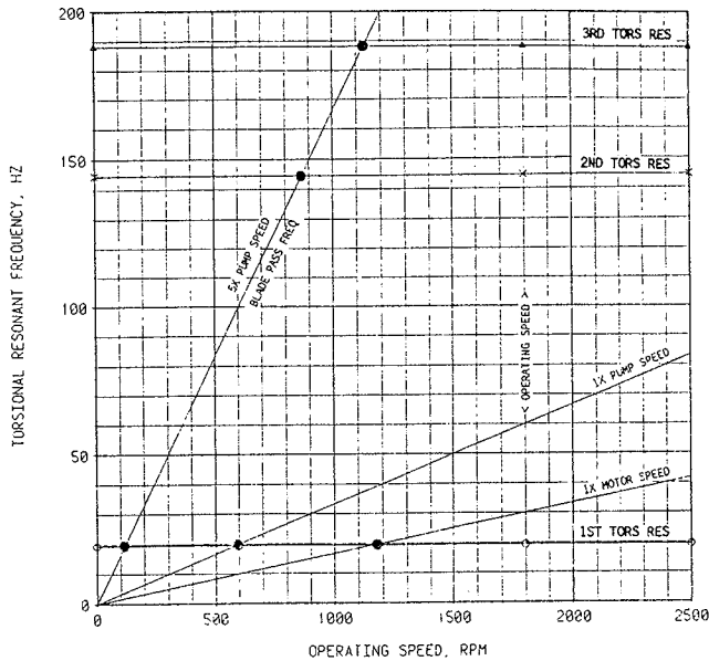
Figure 3. Interference Diagram—Single Speed-Multiple Exciting Orders.
