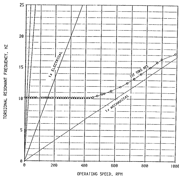
Figure 8. Effect Of Variable Stiffness Coupling on Torsional Natural Frequencies.
