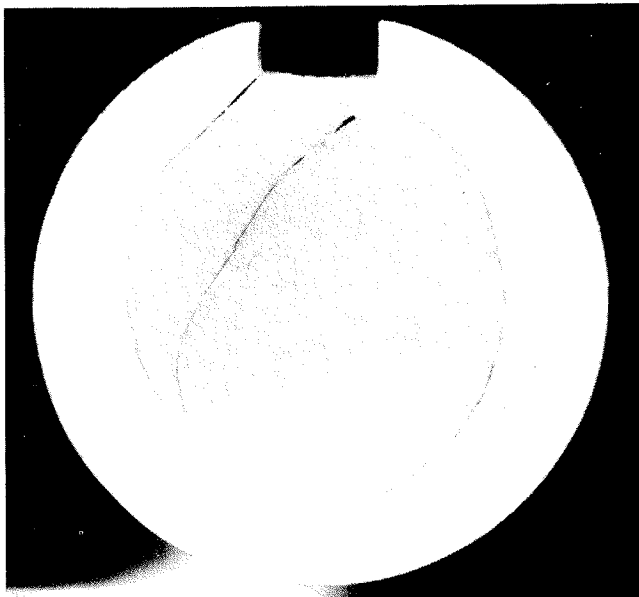
Figure 15. Torsional Failure at Square Cut Keyway.
